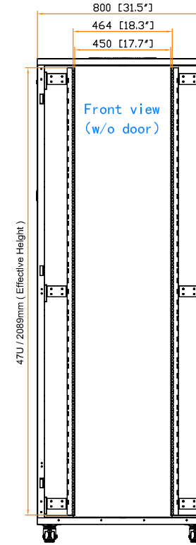
19" rail position
