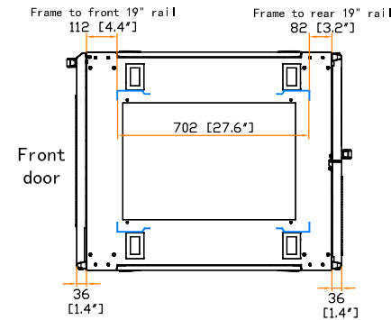
19" rail position
