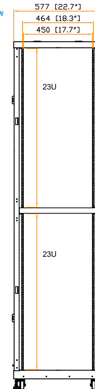
19" rail position
