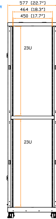
19" rail position
