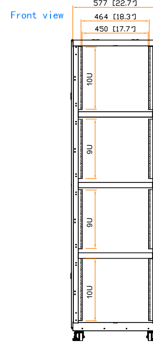
19" rail position
