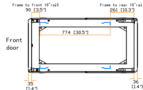
19"rail position
