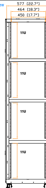
19" rail position
