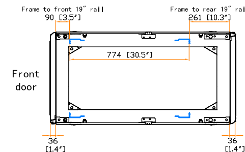
19" rail position
