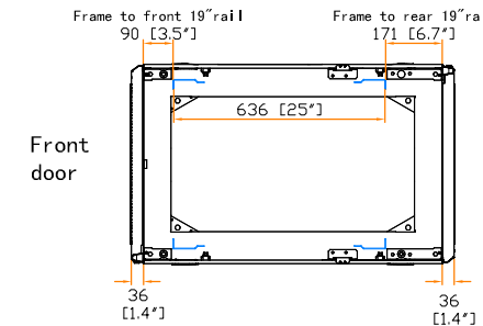
19" rail position
