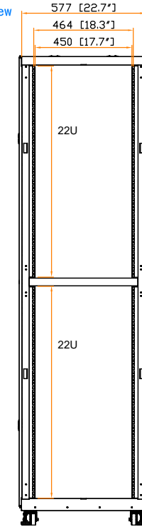
19" rail position
