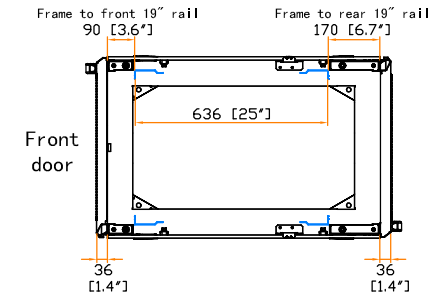
19" rail position
