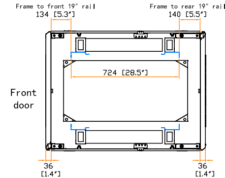
19" rail position
