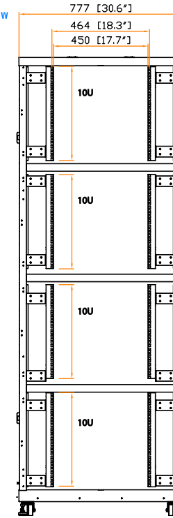
19" rail position
