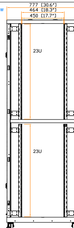
19" rail position
