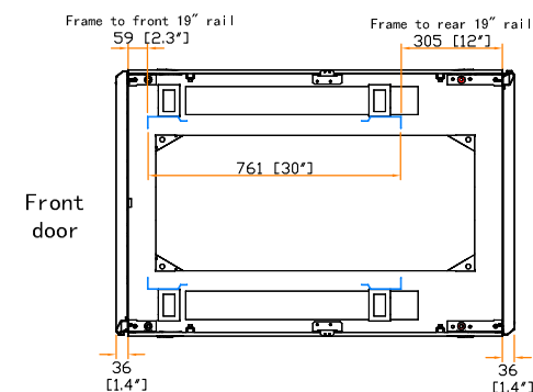
19" rail position
