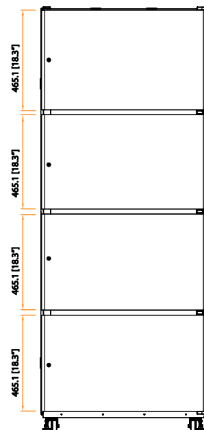
Rear view
