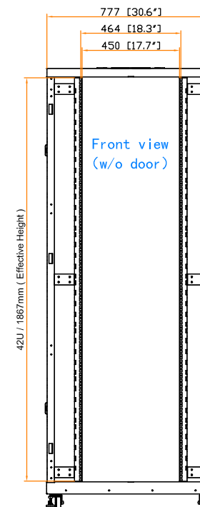
19" rail position
