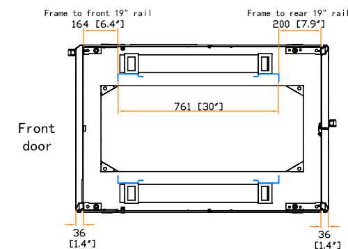
19" rail position
