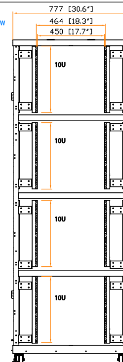
19" rail position
