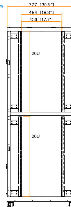
19" rail position
