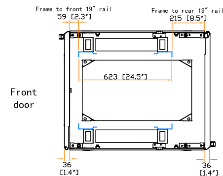
19" rail position
