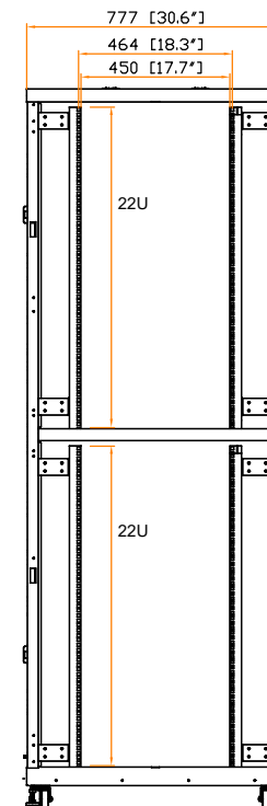
Front view
