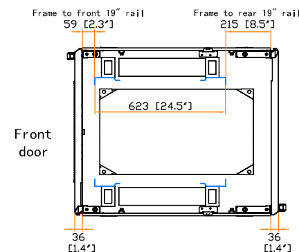
19" rail position
