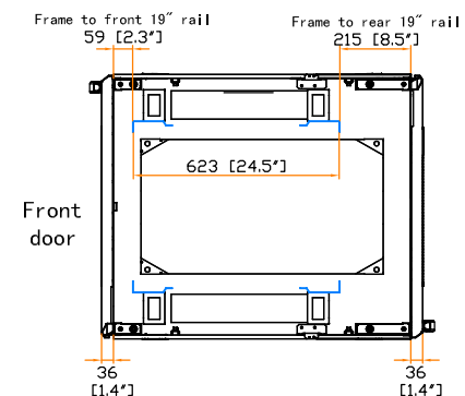
19" rail position
