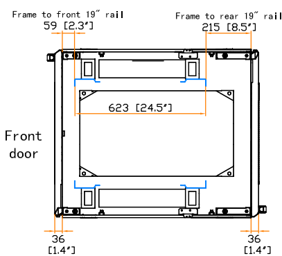
19" rail position
