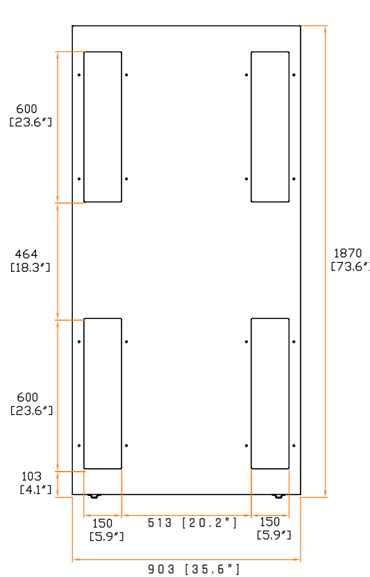
Front view :
