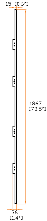
Side view :
