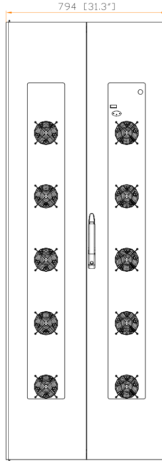
Front view:
