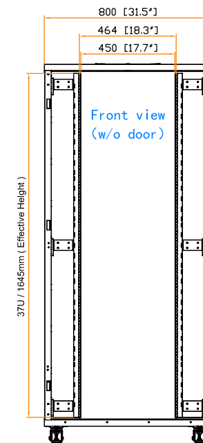
19" rail position
