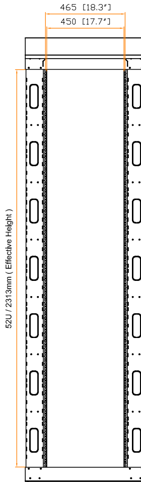
Rear view
