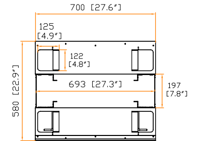
Top view (cable access hole)
