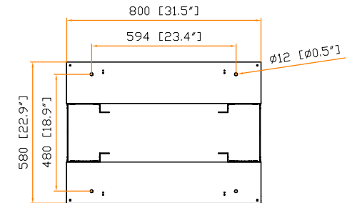
Bottom view (grounding hole position & size)
