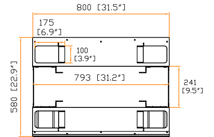
Top view (cable access hole)
