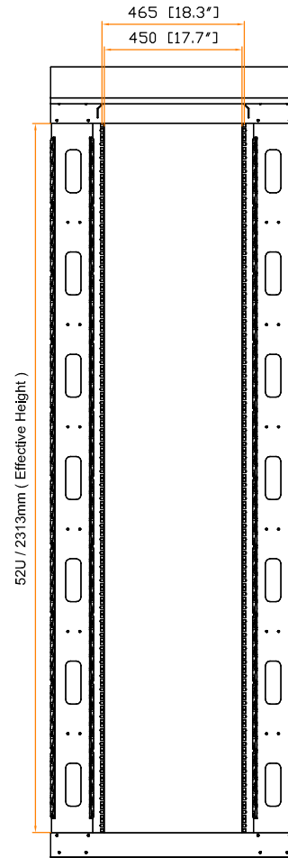
Rear view
