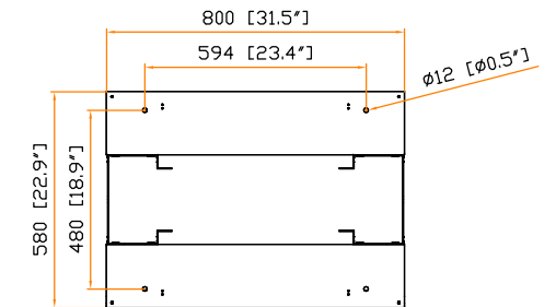
Bottom view (grounding hole position & size)
