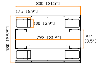
Top view (cable access hole)
