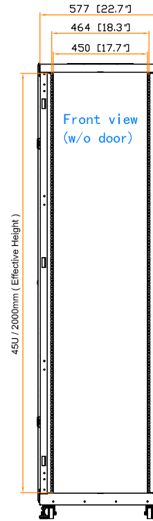
19" rail position
