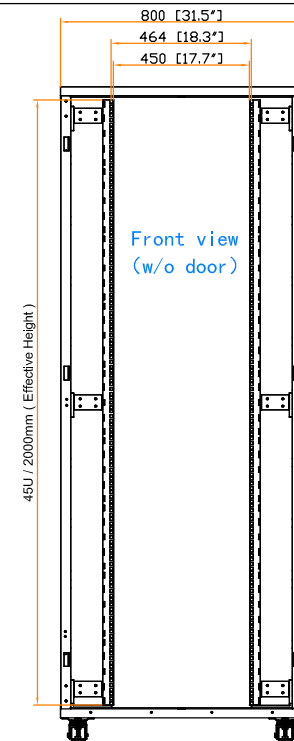
19" rail position
