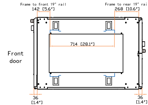
19" rail position
