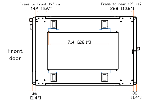
19" rail position
