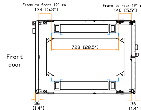
19" rail position
