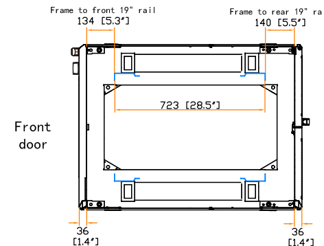
19" rail position
