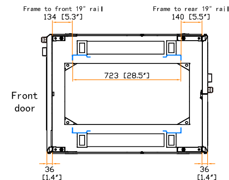
19" rail position
