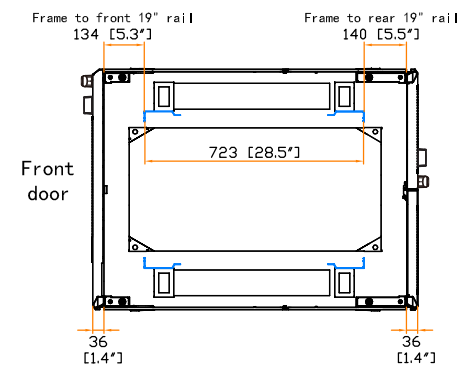
19" rail position
