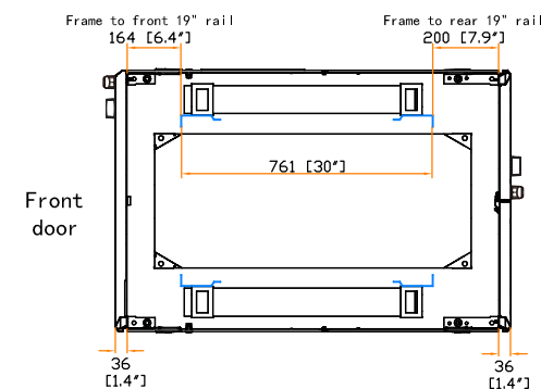
19" rail position
