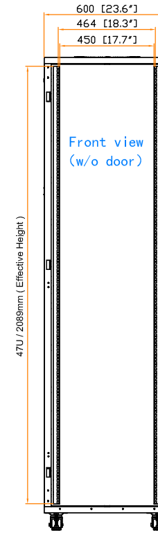
19" rail position
