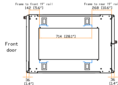
19" rail position
