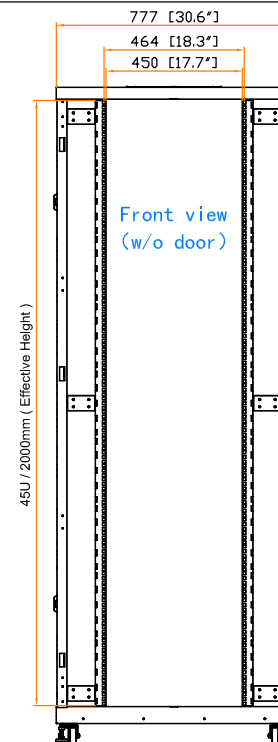
19" rail position
