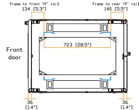
19" rail position
