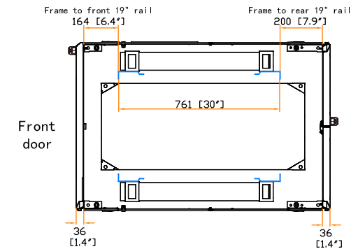
19" rail position
