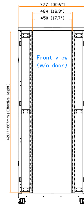
19" rail position
