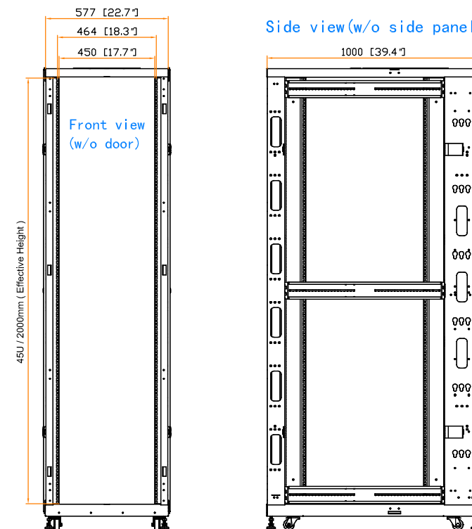
19"rail position
