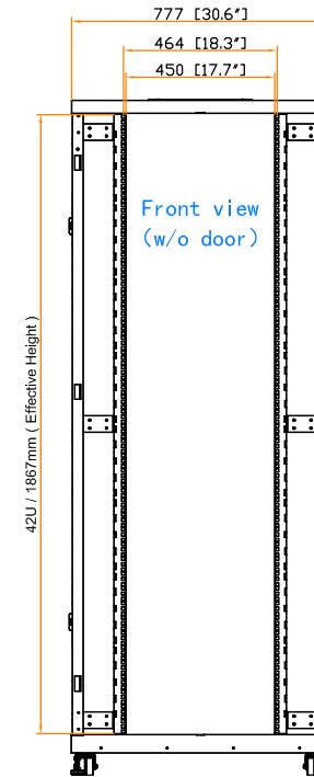
19" rail position
