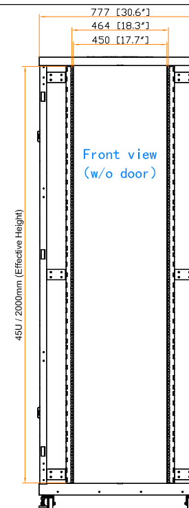
19" rail position
