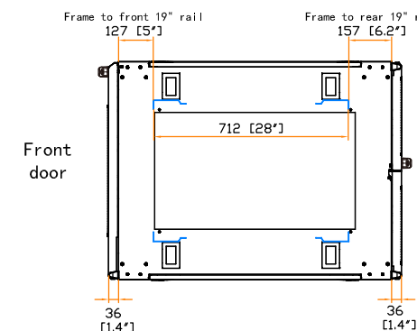
19" rail position
