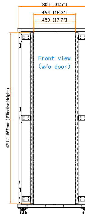
19" rail position
