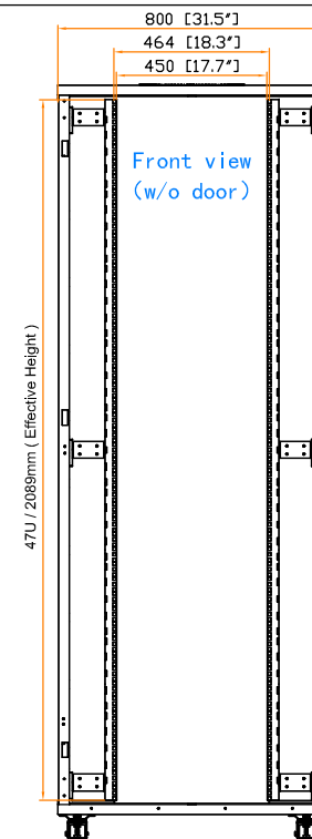
19" rail position
