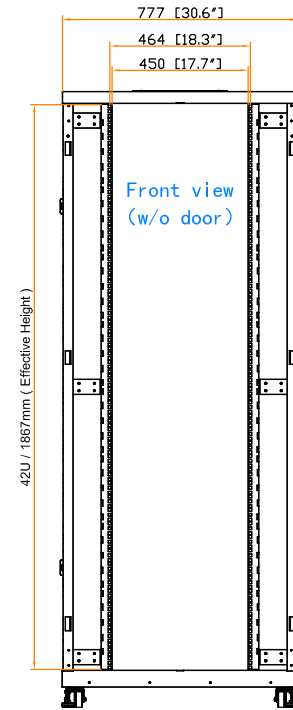
19" rail position
