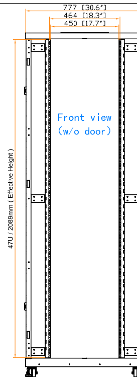
19" rail position
