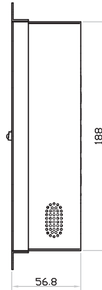
Left-side View
