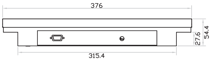
Bottom View
