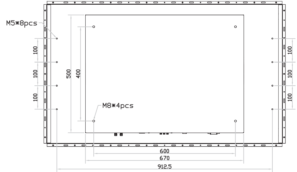
Rear View
