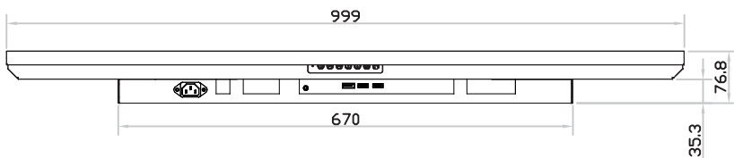
Bottom View
