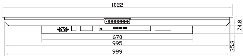
Bottom View
