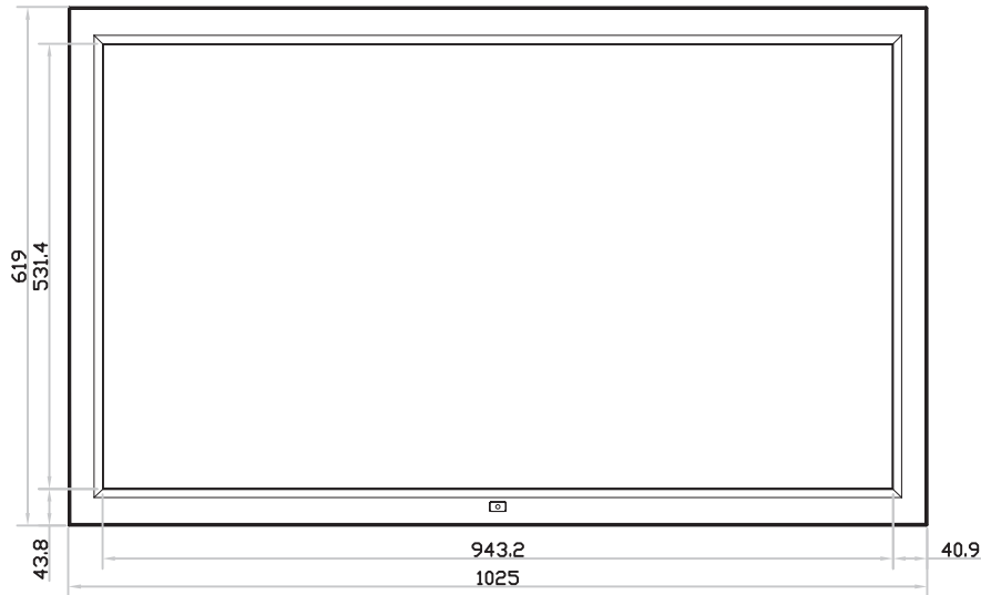
Front View
