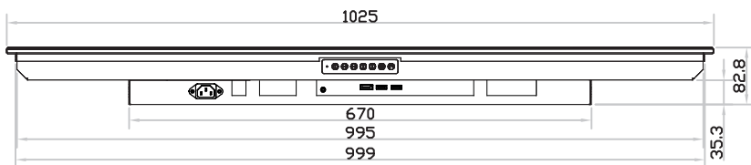
Bottom View
